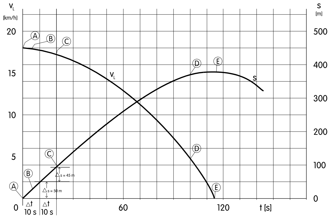
Figure 1: Stopping manoeuvre
